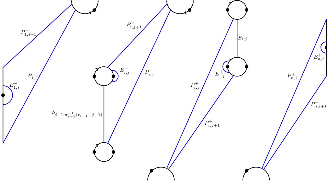
FIGURE 10. Functors from \mathcal{W}(0;3) and \mathcal{W}(0;4) corresponding to embeddings of disks
